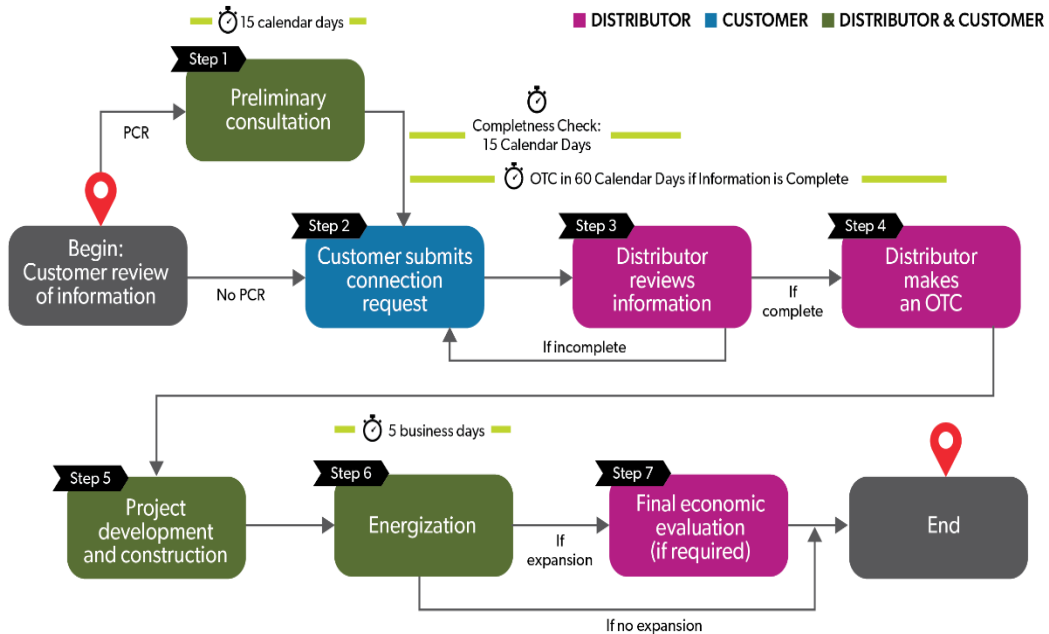
Figure 1: High-level process flow for an EVSE connection
